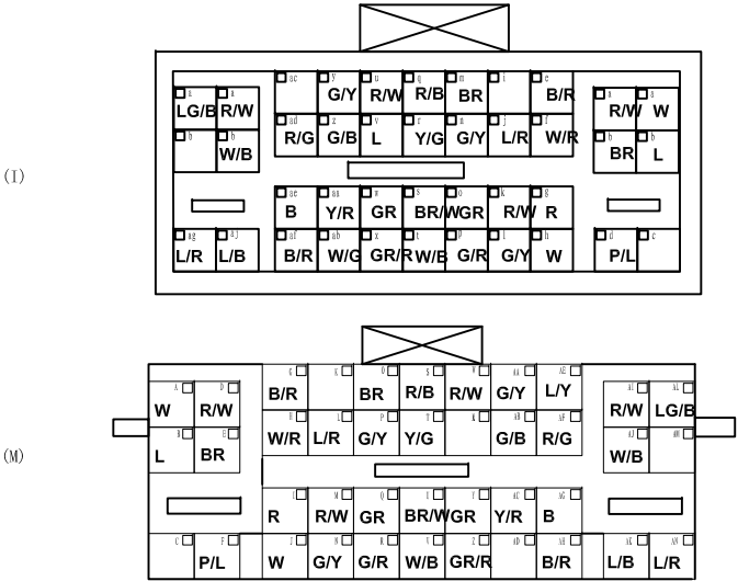
X-11 仪表线束 (I) - 中部线束 (M)
